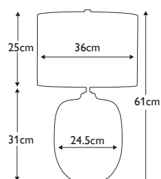
30236 1 lt Table Lamp Base: Light Grey to Snow White fade ceramic Shade: Ivory Faux Silk Max. Wattage: 1 x 60W E27
