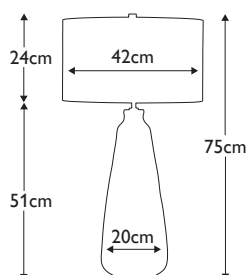
30378 1 lt Table Lamp Base: Sage Green ceramic Shade: White Faux Silk Max. Wattage: 1 x 60W E27
